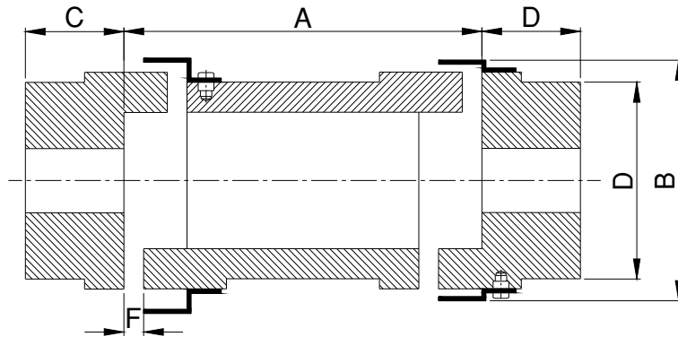
EXTERNAL SPIDER ALUMINIUM SPACER COUPLING
