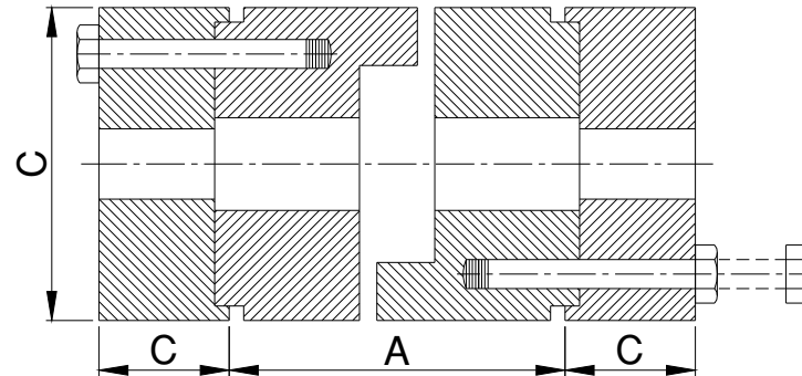
STANDARD SPACER COUPLING
